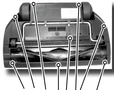
Remove 8 Torx Screws
